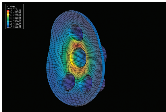
Von Mises stresses at the surface of the cement layer, which bonds the implant to the bone.
